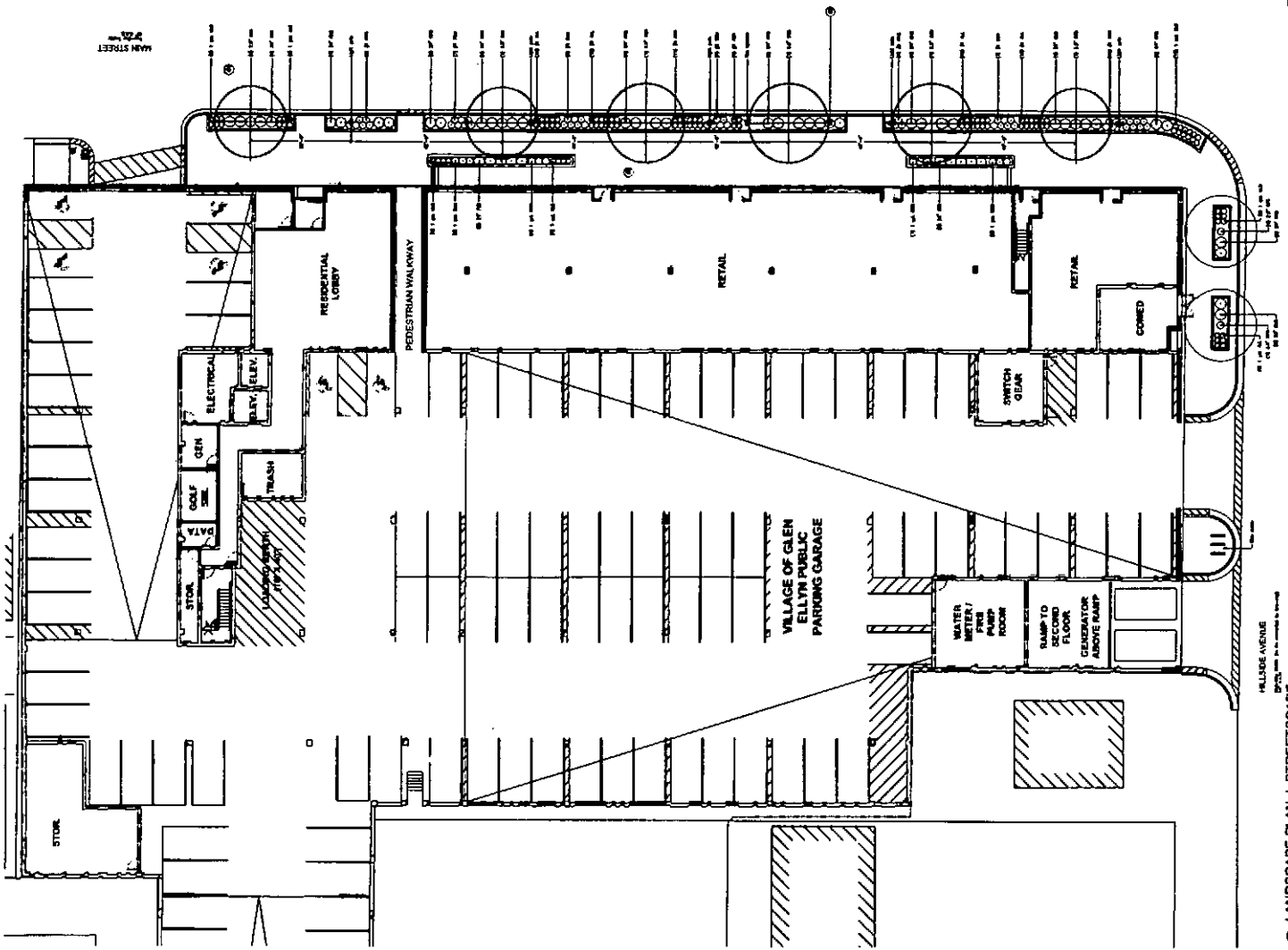
1 LANDSCAPE PLAN | STREETSCAPE 1/8" = 1'-0"
